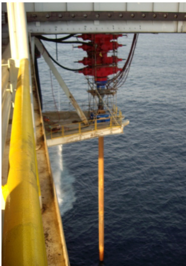
Typical conductor installation
