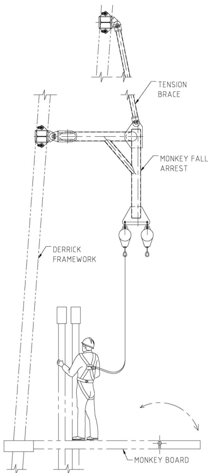
General Arrangement
