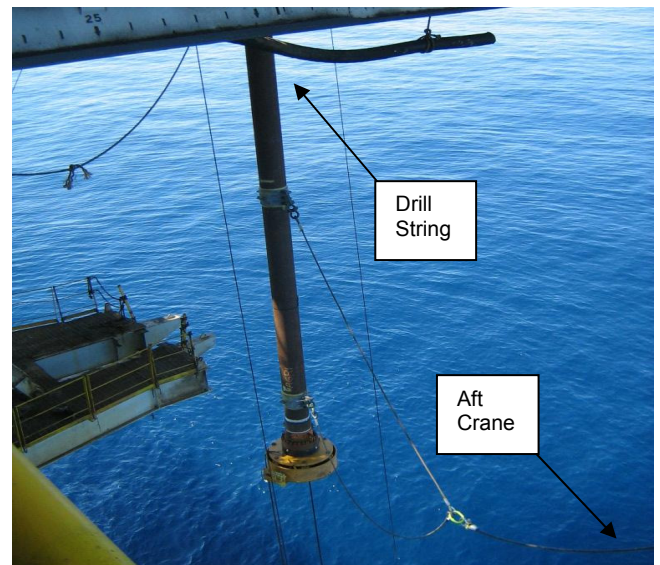
Handshake lift of 22" HP riser
