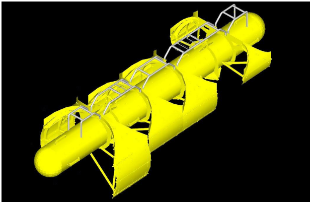
Mid Water Arch – CAD Model
