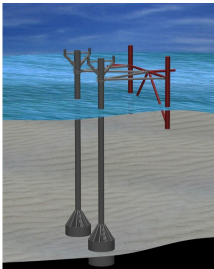
Conceptual Sketch of Annexe (MSF & BR-A not shown for clarity)
