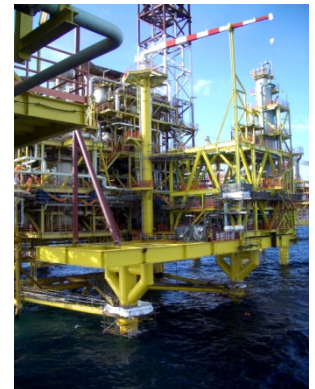
BRA Annexe installed with first process module in place
