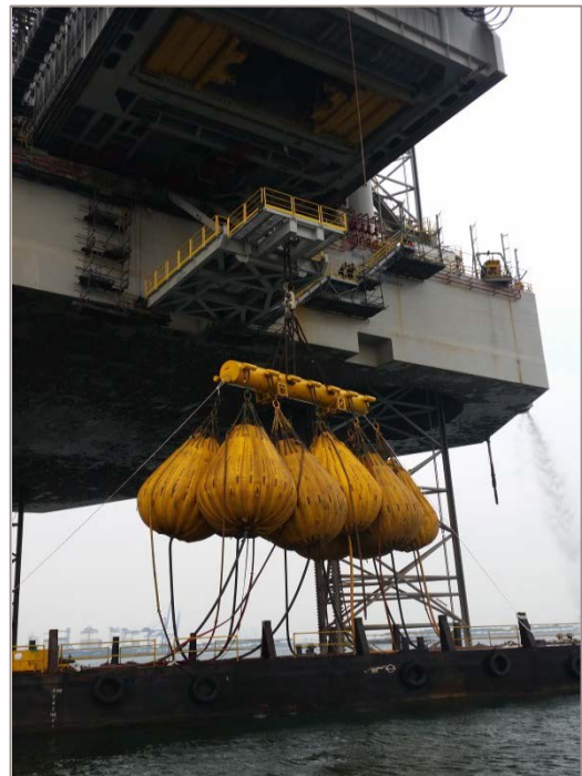
Tension Deck under 450Te load test
