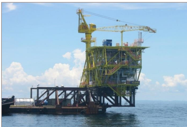
WP-PA Topsides Marine Transport – Jacking Position
